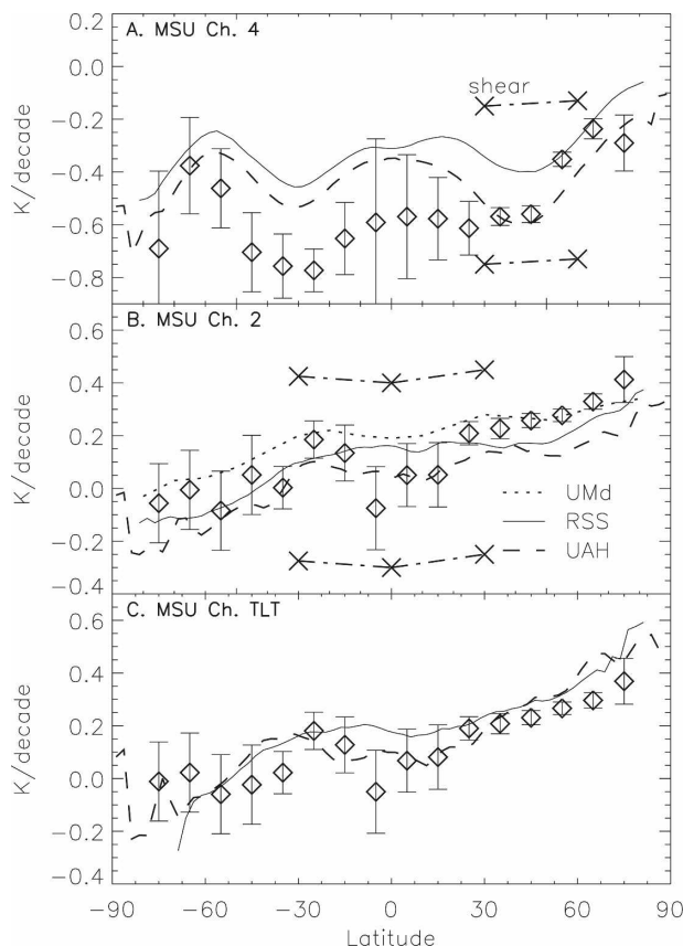
FIG. 4. Comparison of trends, 1979–2005. Lines show MSU channels (a) 4, (b) 2, and (c) TLT linear trends from RSS (solid) channel 2, version 3.0 (Mears et al. 2003)/TLT version 5.0 (Mears and Wentz 2005); UAH (dashed) TLT version 5.2/channel 2, version 3.0 (Christy et al. 2003); and UMD (dotted, channel 2 only; Vinnikov et al. 2006). Symbols show simulated MSU trends from round 3 averaged over the two detection schemes, with approximate 1-sigma error bars, based on the median trend at each pressure from stations at that latitude. The differences in vertical position of two crosses joined by dot-dashed lines show the meridional differences between the trend at the two latitudes implied by that of wind shear via thermal wind balance. Their vertical positions are arbitrary.
