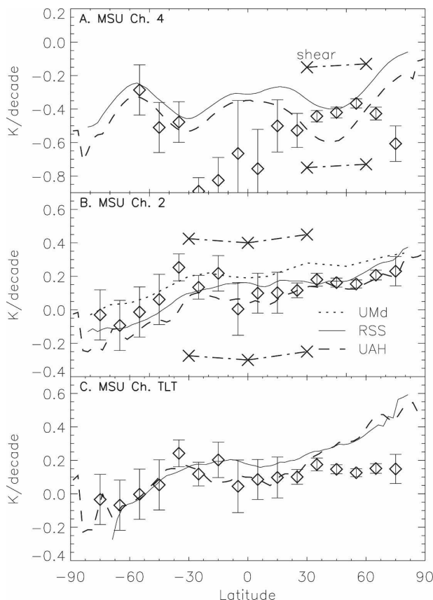
FIG. 5. As in Fig. 4, but for unadjusted data.
