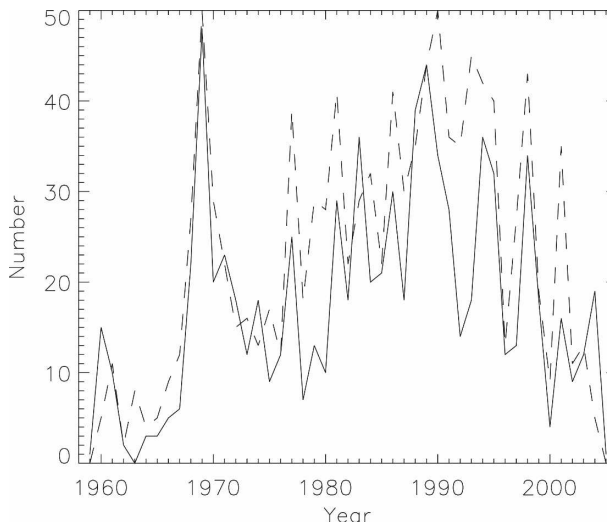
FIG. 2. Number of detected T changepoints per year with two-phase regression (solid) and L96 (dashed) methods, among group A stations at round 3.
