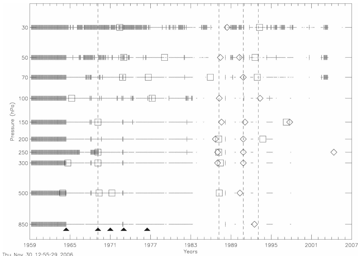
FIG. 1. Results of changepoint detection at Niamey Aerodrome in Niger (WMO 61052) with the L96 scheme. Diamonds and squares represent LCPs found in rounds 1 and 2, respectively, and vertical dashed lines show locations of final CPs. Vertical hatching by level shows months with insufficient data, while small dots show months with sufficient data at only one time of day. Solid triangles at bottom show times of CPs detected by LKS at this station at 300 hPa.
