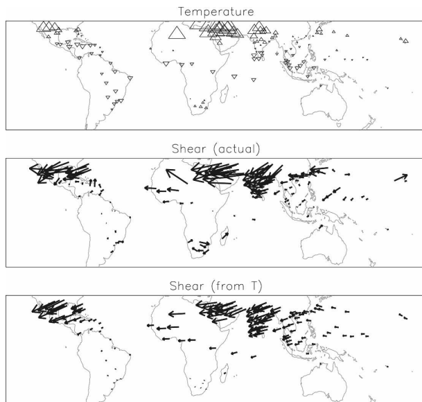
FIG. C1. (a) Temperature, (b) vertical shear, and (c) estimated thermal wind vertical shear loadings of the leading mode for JJA in the tropics. Triangle sizes are proportional to the temperature magnitude and point up or down for positive or negative loading, respectively; arrow lengths are proportional to shear \times f , where f is the Coriolis parameter.
